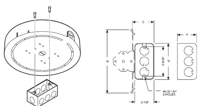
Type B: 2-gang handy box/switch box
